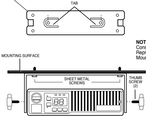
Figure 4. Trunnion Mount for Radio
